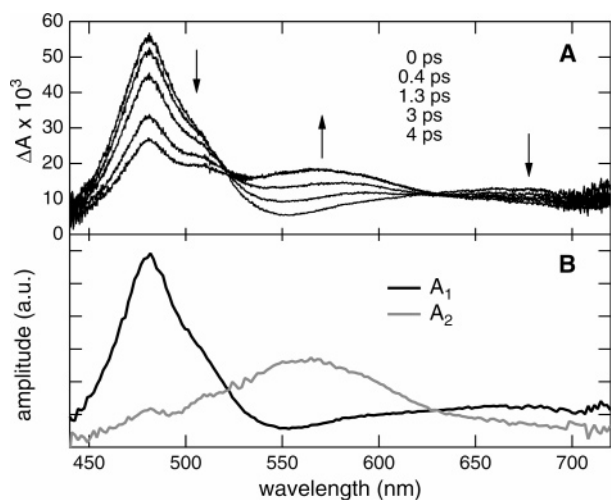
Figure 8. (A) TA spectra recorded at different time delays after 400 nm excitation of NPe in ACN; (B) spectral dependence of the amplitude factors obtained from global analysis (see text).
